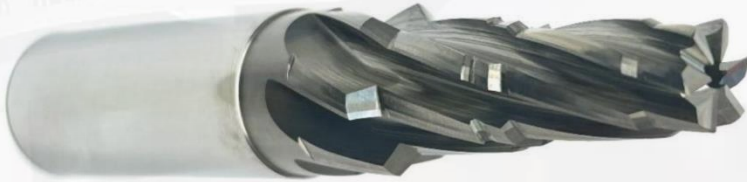
6 FLUTE MULTI-STEP CUTTER WITH COOLANT HOLE
